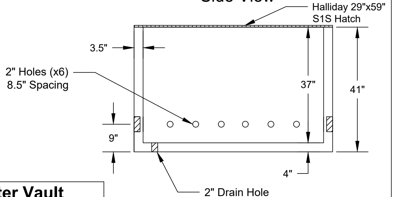
Side View
