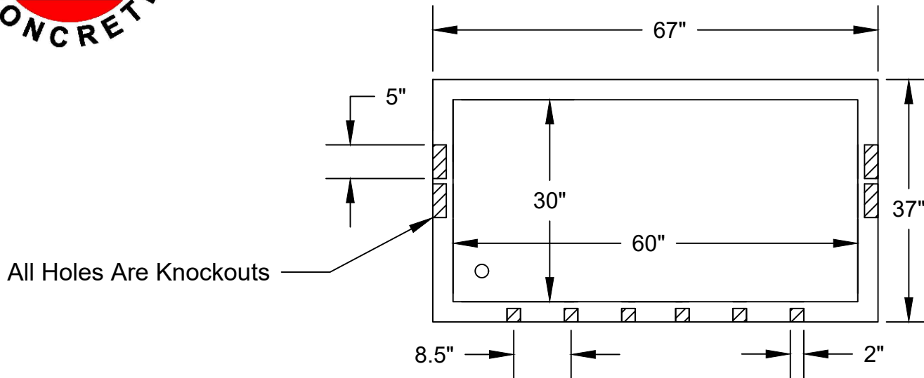
End View
